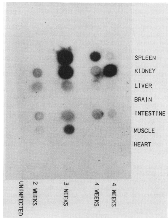
FIG. 3. Representative sample of results of dot blot hybridization used to detect SBR virus RNA in organs of experimentally infected rainbow trout fingerlings. ^{32}\text{P} -labeled probes from the clone 33 insert were hybridized with nucleic acids extracted from different organs as described in the text. Nucleic acids extracted from organs of one representative fish sacrificed 2 weeks postinfection, one fish sacrificed 3 weeks postinfection, and two fish sacrificed 4 weeks postinfection were used to show viral RNAs in spleen and kidney tissues. Nucleic acids extracted from organs of one sham-inoculated fish after 4 weeks were used as a control.
