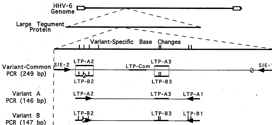
FIG. 1. Diagram of primers and probes. Arrow, primer; short horizontal thick lines, probes; hatched circles, TaqI sites.
