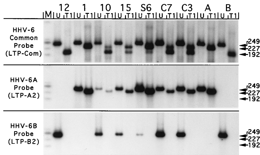
FIG. 2. Autoradiogram of hybridized PCR products from selected amplification reactions. Lanes contain undigested (U) or TaqI -digested (T1) products or ^{32} P-end-labeled \phi X173 Hae III-cut DNA size markers (M). Each pair of undigested and digested PCR products is designated as in Table 1. A and B, prototype HHV-6 variants A (U1102) and B (Z-29), respectively. Products from each amplification reaction were hybridized with a variant-common probe (LTP-Com), variant A-specific probe (LTP-A2), or variant-B specific probe (LTP-B2). The full-length SIE-1/2 variant-common product appears at 249 bp (all three panels), the TaqI -digested variant A product appears at 227 bp (top and middle panels), and the TaqI -digested variant B product appears at 192 bp (top panel). TaqI digestion abrogates hybridization of the variant B probe with variant B PCR products, as shown in the bottom panel and predicted by the diagram in Fig. 1.
