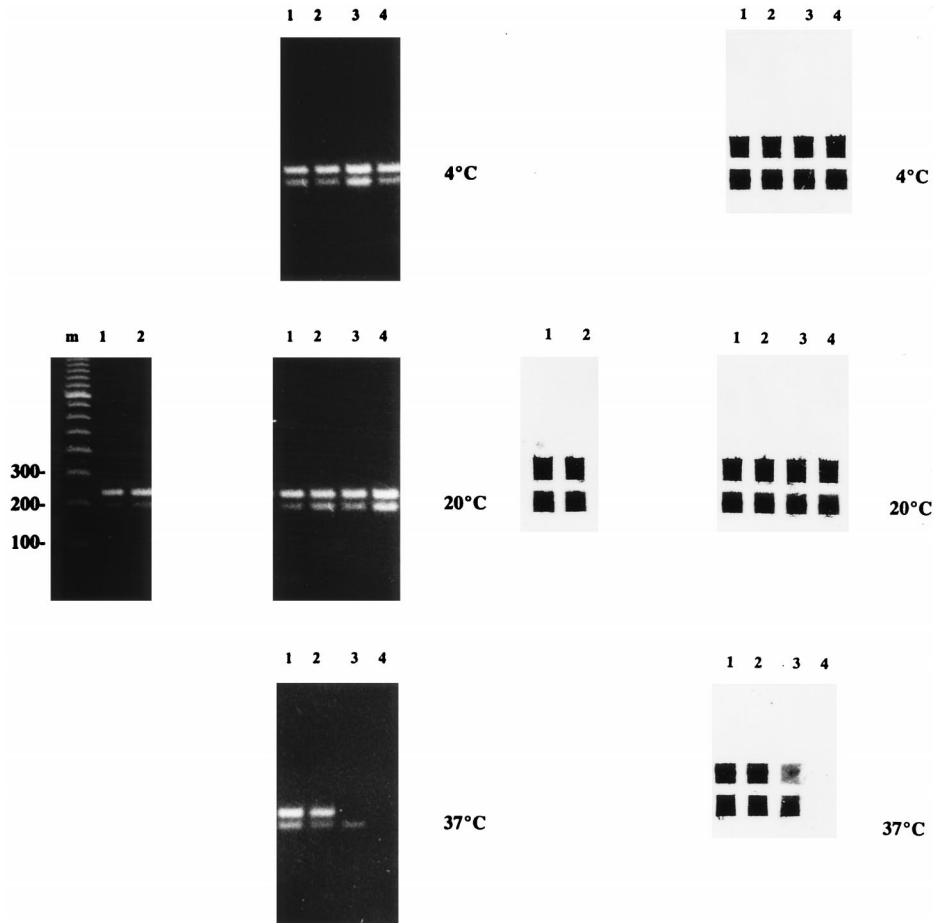
FIG. 2. Gel electrophoresis (left) and reverse cross-blot hybridization (right) results of the reconstituted PCR mixes after storage. The freeze-dried PCR mixes were stored for 3 months (lanes 1 and 2) and 1 year (lanes 3 and 4) at different temperatures as indicated and, upon reconstitution, were tested with 500 (lanes 1 and 3) and 50 (lanes 2 and 4) fg of purified M. bovis BCG DNA. The photographs at the left in each panel show the results for PCR mixes reconstituted directly after freeze-drying. Lane m contains a 100-bp ladder (Pharmacia) as a molecular weight marker; the 100-, 200-, and 300-bp fragments are indicated. Reverse cross-blot hybridization was done with probe Pt3 to capture the 249-bp IS6110 PCR products (top wells) and pTub1 to capture the 208-bp 16S rDNA PCR products (bottom wells).
