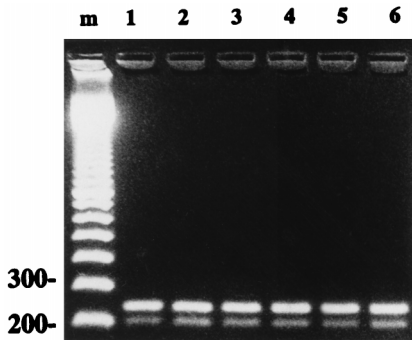
FIG. 1. Effect of trehalose on the performance of PCR with M. bovis BCG DNA. A gel electrophoresis analysis of PCR performed with the addition of trehalose at concentrations (% [wt/vol]) of 0 (lane 1), 2 (lane 2), 4 (lane 3), 6 (lane 4), 8 (lane 5), and 10 (lane 6) to the PCR mix shows the 208-bp (16S PCR product) and 249-bp (IS6110 PCR product) bands. Lane m contains a 100-bp ladder (Pharmacia) as a molecular weight marker; the 200- and 300-bp fragments are indicated.
