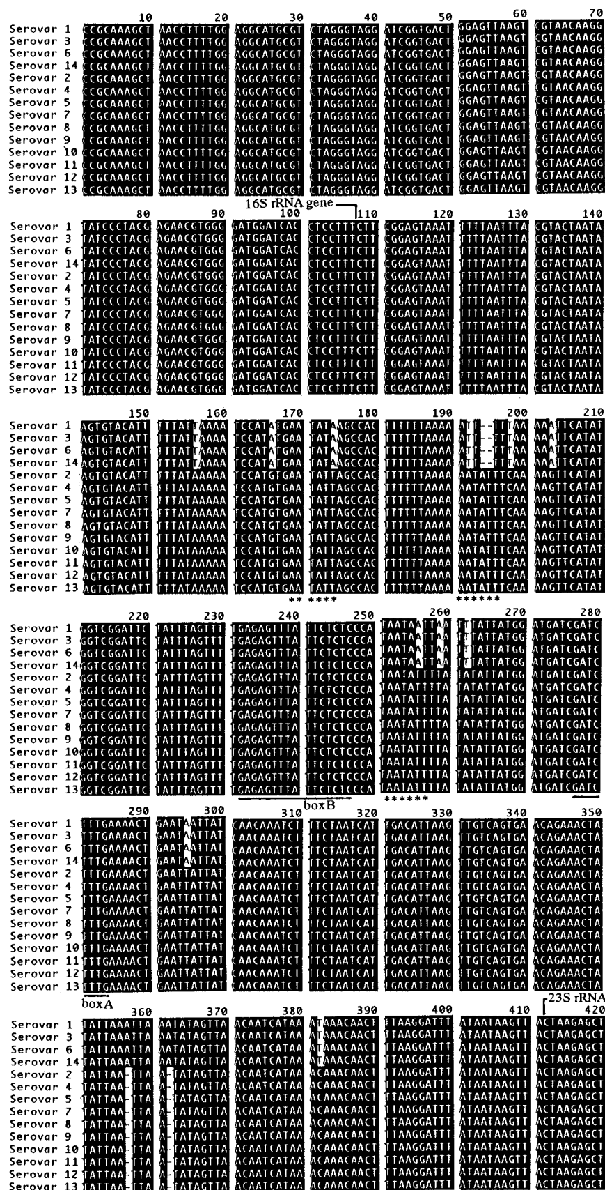
FIG. 1. Sequence alignment for the 14 strains from the 14 serovars of U. urealyticum . The nucleotide sequence numbers are given from a consensus alignment. Nucleotides that are identical in two out of three sequences are shown as white letters on a black background. Dashes indicate spacers between adjacent nucleotides introduced for maximum alignment. Box A and box B are underlined. Three SspI (5'-AATATT-3') sites on the T960 biovar sequences are indicated by asterisks.
