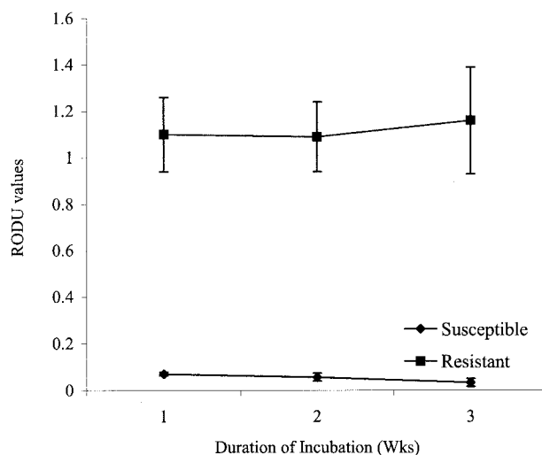
FIG. 2. Growth patterns of rifampin-susceptible ( n = 37 samples in the first week, 56 in the second week, and 58 in the third week) and rifampin-resistant ( n = 6 in the first week and 8 in the subsequent weeks) strains of M. tuberculosis as reflected by RODU values (means \pm standard errors) [(RODU = OD 570 of rifampin-containing medium)/(OD 570 of drug-free medium)]. The difference in RODU values in each week was statistically significant ( P < 0.01 [Mann-Whitney test]).
