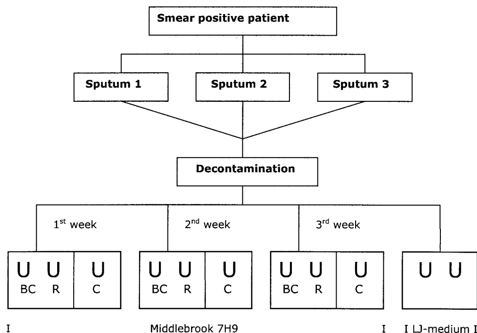
FIG. 1. Flow chart of MTT assay. Abbreviations: BC, bacterial control without rifampin; R, tube with 2 \mu g of rifampin/ml; C, control without bacteria. LJ, Löwenstein-Jensen.
