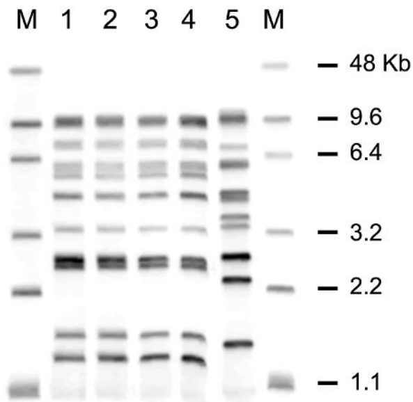
FIG. 1. Ribotyping for serotype Panama isolated from the infant and from breast milk of the mother. Lane 1, isolate from blood; lane 2, isolate from CSF; lane 3 and 4, breast milk isolates from two different periods; lane 5, Salmonella enterica serotype Infantis (ATCC 51741). M, marker lane.
