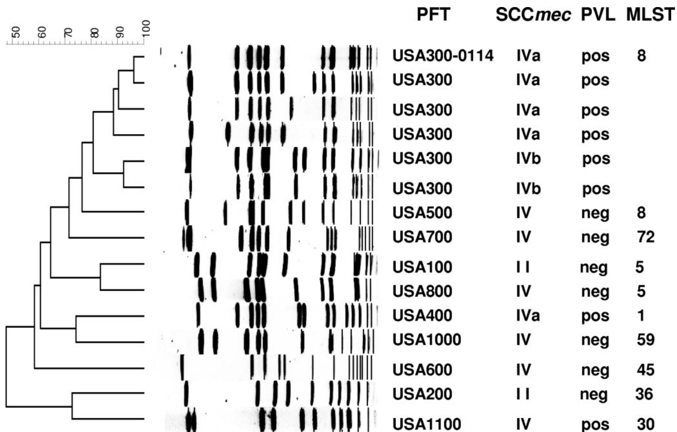
FIG. 1. PFGE profiles of SmaI macrorestriction patterns of S. aureus isolates of various USA types (Centers for Disease Control and Prevention, unpublished data); 46). PFTs, SCCmec types, results of the PCR assay for PVL toxin genes (pos, positive; neg, negative), and sequence types determined by MLST are shown.
