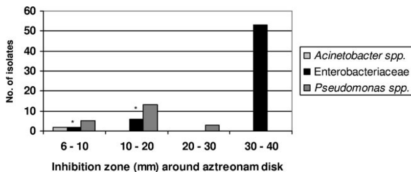
FIG. 3. Inhibition zone diameters (in millimeters) around the aztreonam disk (30 \mu g) for the 84 metallo- \beta -lactamase-carrying isolates. Asterisks indicate Enterobacteriaceae isolates ( n = 8 ) found to produce an AmpC-type or extended-spectrum \beta -lactamase.
