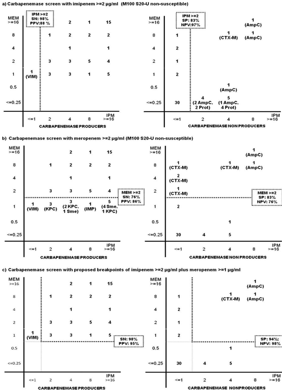
FIG. 1. Scattergrams showing numbers of isolates at the indicated carbapenem MICs (averages of duplicate values, in \mu\text{g/ml} , of imipenem [IPM] and meropenem [MEM]) obtained by Vitek 2 for carbapenemase producers and carbapenemase nonproducers. (a) The sensitivity (SN), specificity (SP), positive predictive value (PPV), and negative predictive value (NPV) were calculated for carbapenemase screening using the imipenem M100-S20-U CLSI nonsusceptibility breakpoint (a MIC of \geq 2 \mu\text{g/ml} ) (members of the Proteaeae tribe were excluded from the group of carbapenemase nonproducers for the calculation of SP, PPV, and NPV). (b) Meropenem M100-S20-U CLSI nonsusceptibility breakpoint (a MIC of \geq 2 \mu\text{g/ml} [dashed lines]). (c) Cutoff values recommended in this work for a combination of imipenem (MIC \geq 2 \mu\text{g/ml} ) and meropenem (MIC \geq 1 \mu\text{g/ml} ). The mechanisms of resistance are indicated for undetected carbapenemases or isolates with interfering mechanisms. Prot, Proteaeae ; CTX-M, production of the CTX-M-2 ESBL plus porin loss; AmpC, derepressed expression of chromosomal cephalosporinase plus porin loss.
