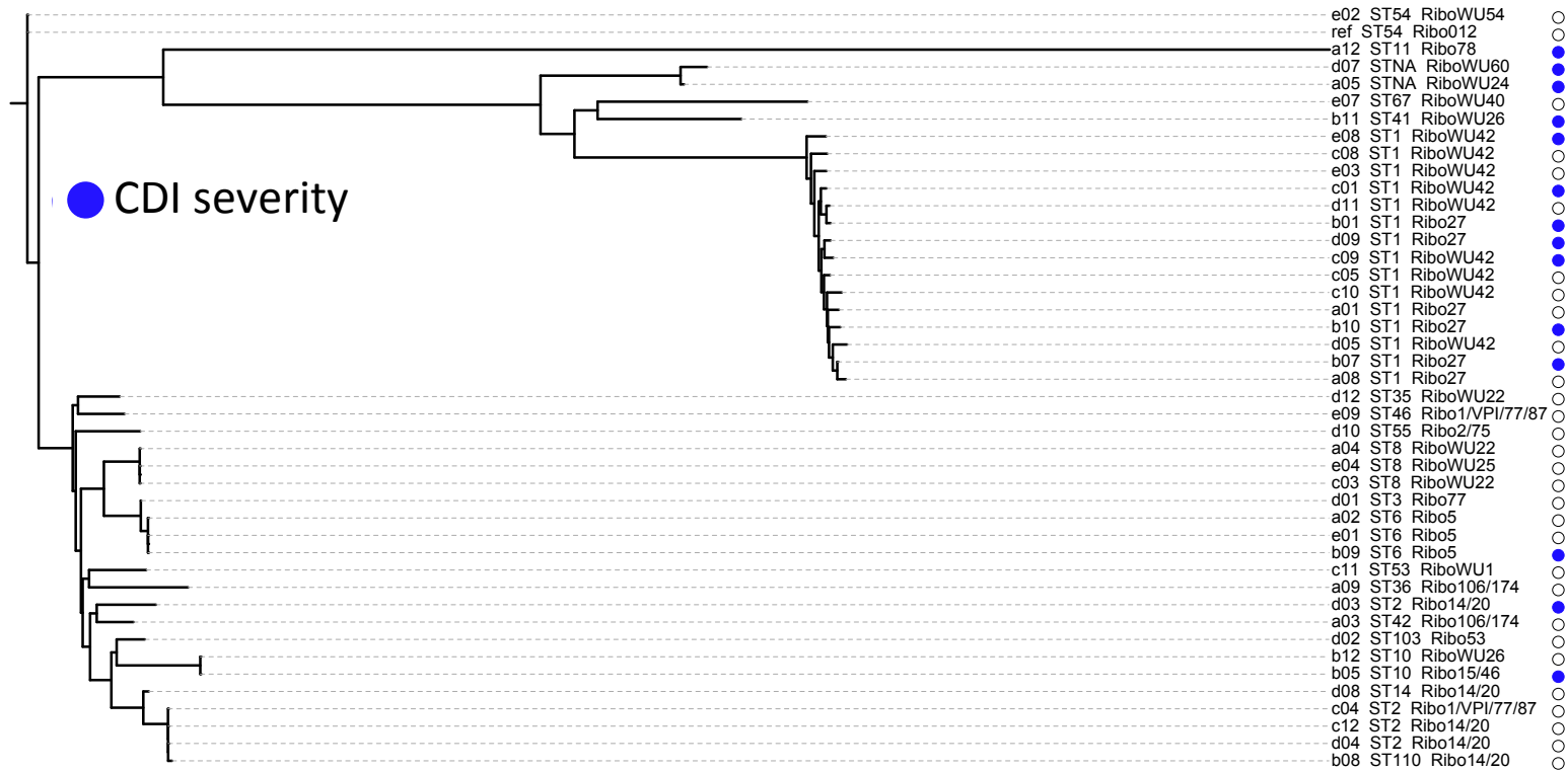
Fig S1. Phylogenetic tree of the 46 C. difficile strains based on the PaLoc SNPs. The tree was built in a similar manner from the SNPs in PaLoc. The tree is annotated by disease severity.
